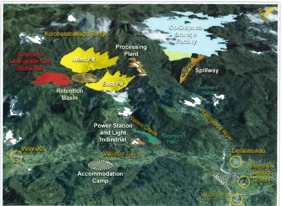
Co-Disposal Storage Facility
